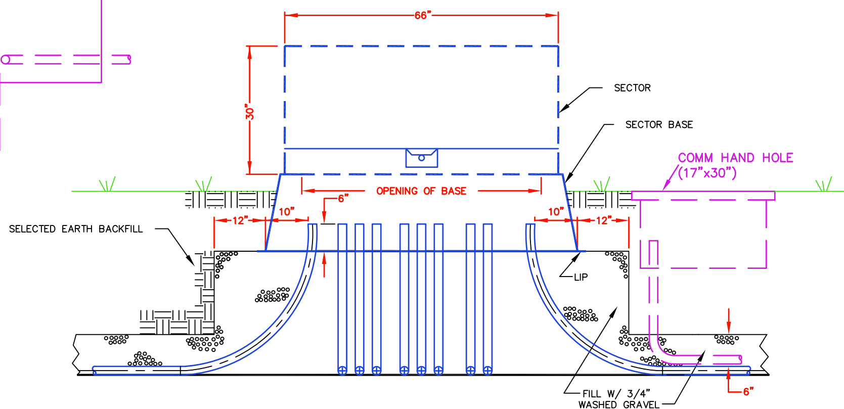
SECTOR FRONT ELEVATION
