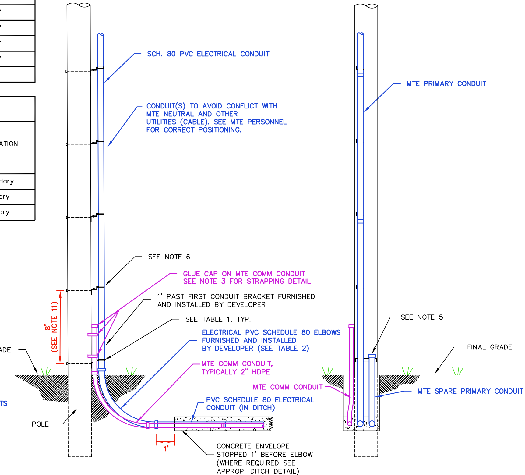
SIDE ELEVATION
