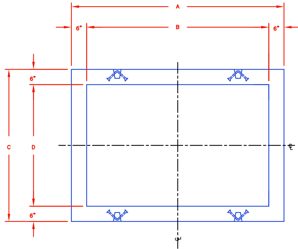
PLAN VIEW
