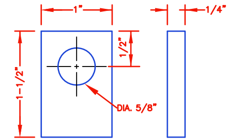
GROUND TAB
