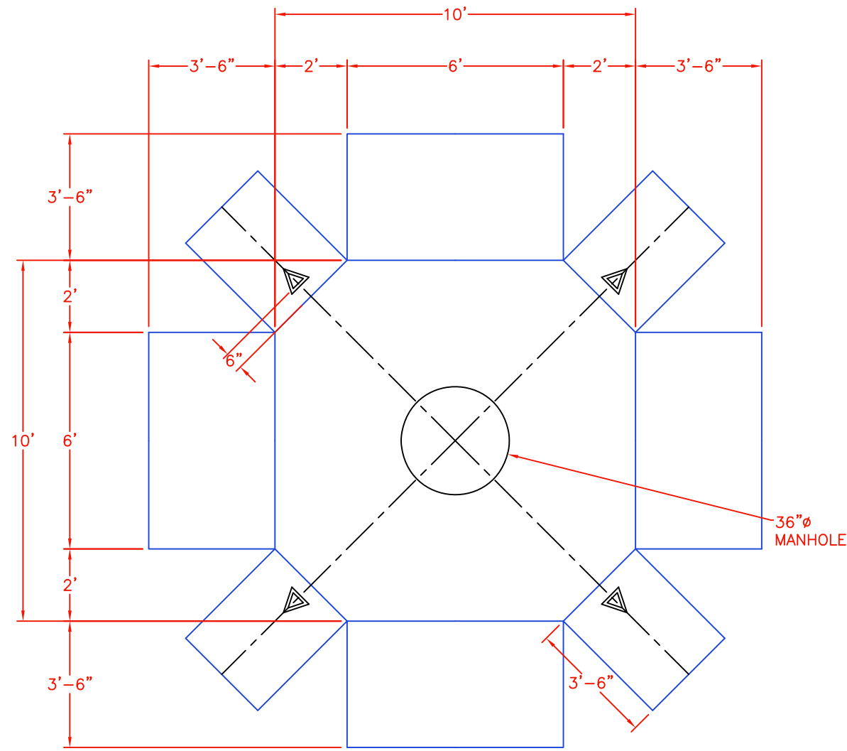
TOP VIEW
