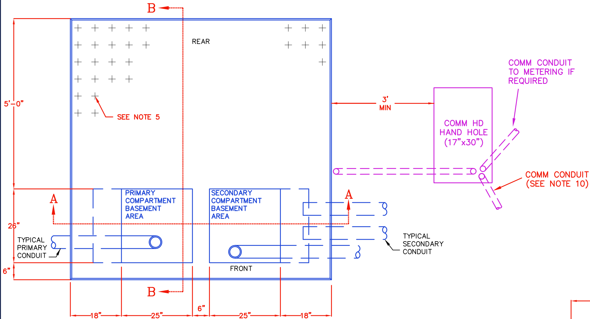
PLAN VIEW
