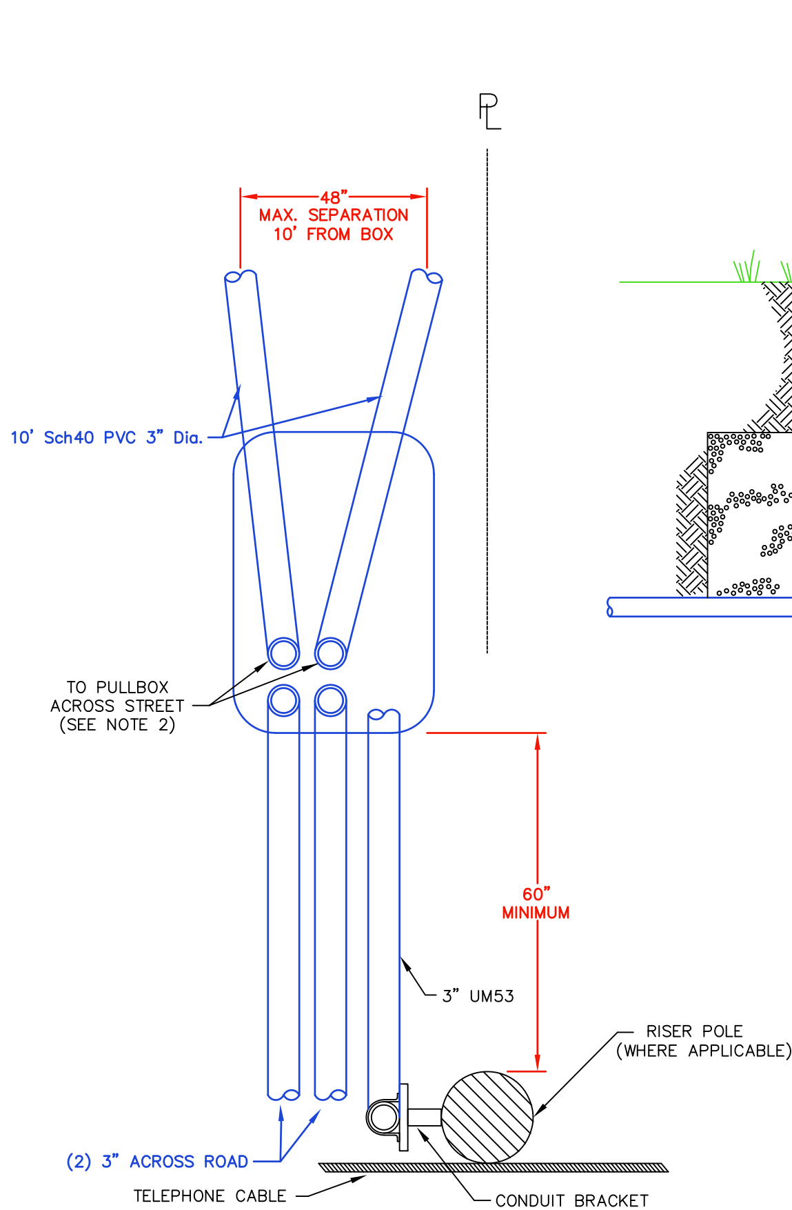
PLAN VIEW SCALE: NONE
