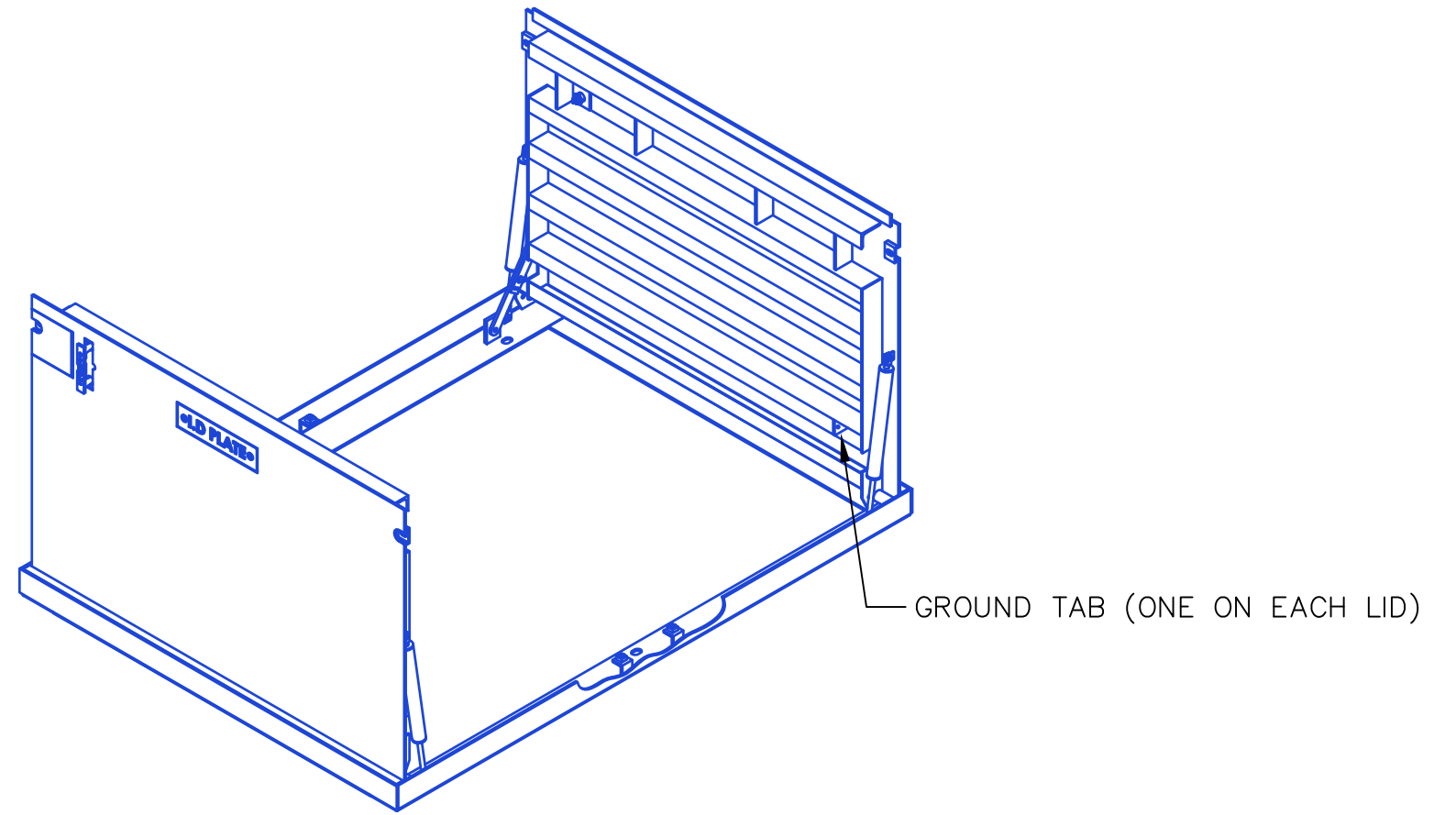
VAULT COVER ISOMETRIC VIEW
