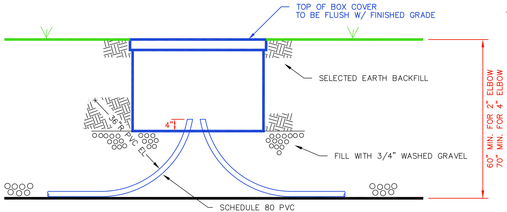
SIDE VIEW
