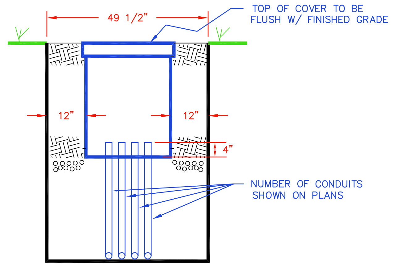
END VIEW
