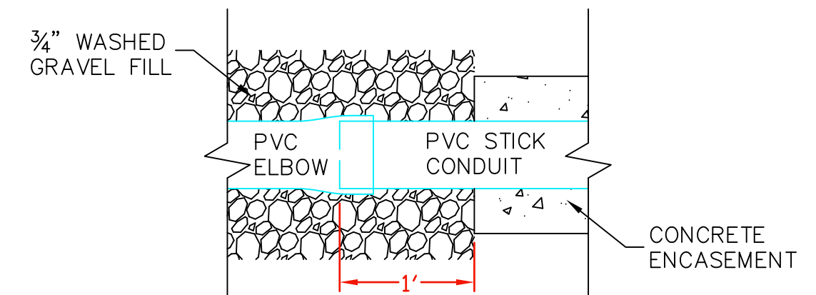
ELBOW TO STICK TRANSITION DETAIL
