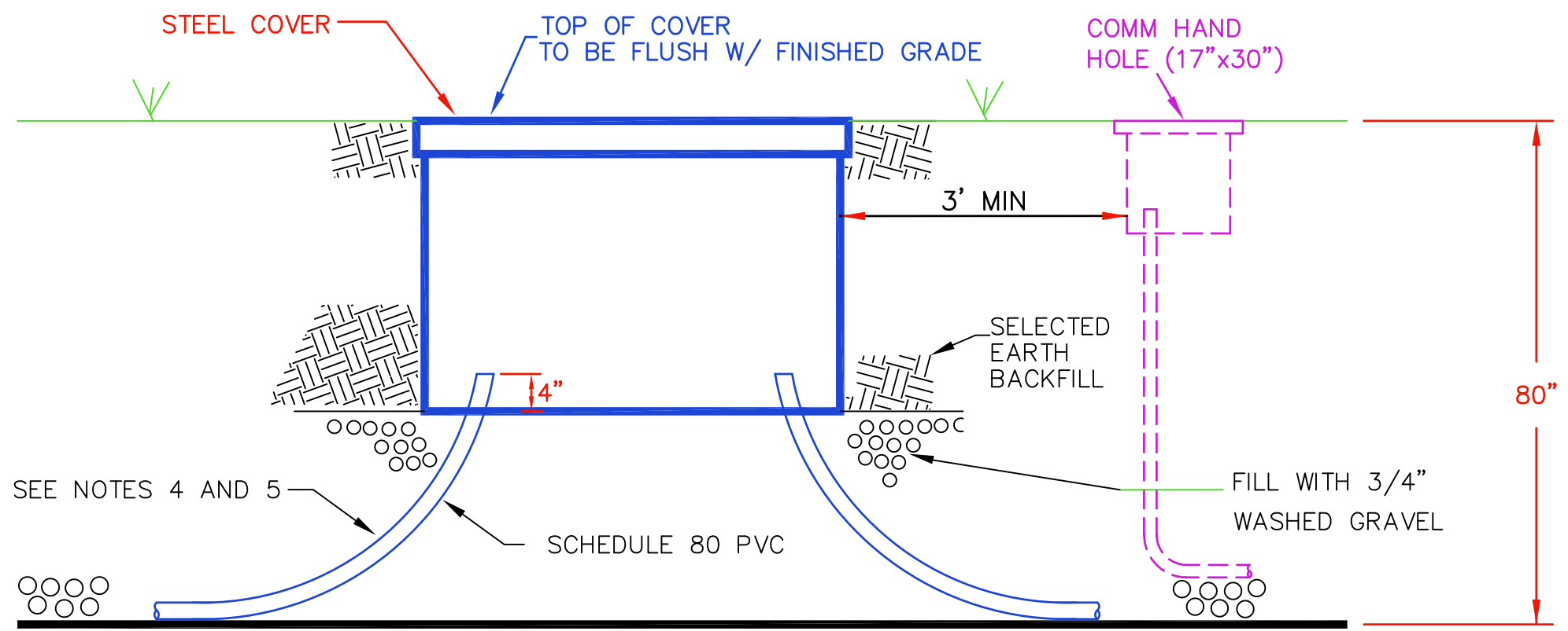
SIDE VIEW
