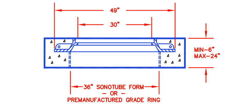
MANHOLE THROAT AND COVER DETAIL
