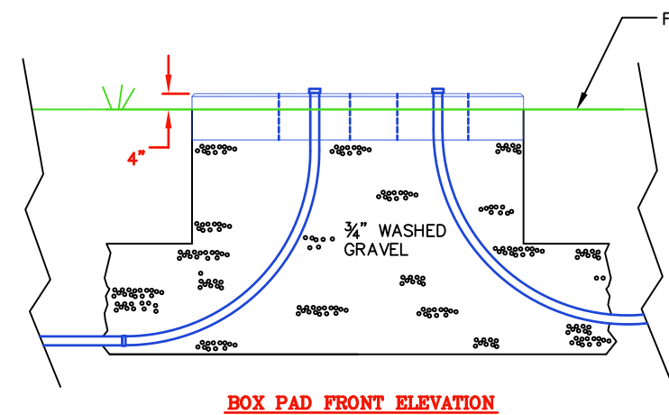
EXISTING SECTOR SIDE ELEVATION BOX PAD FRONT ELEVATION SIDE VIEW
