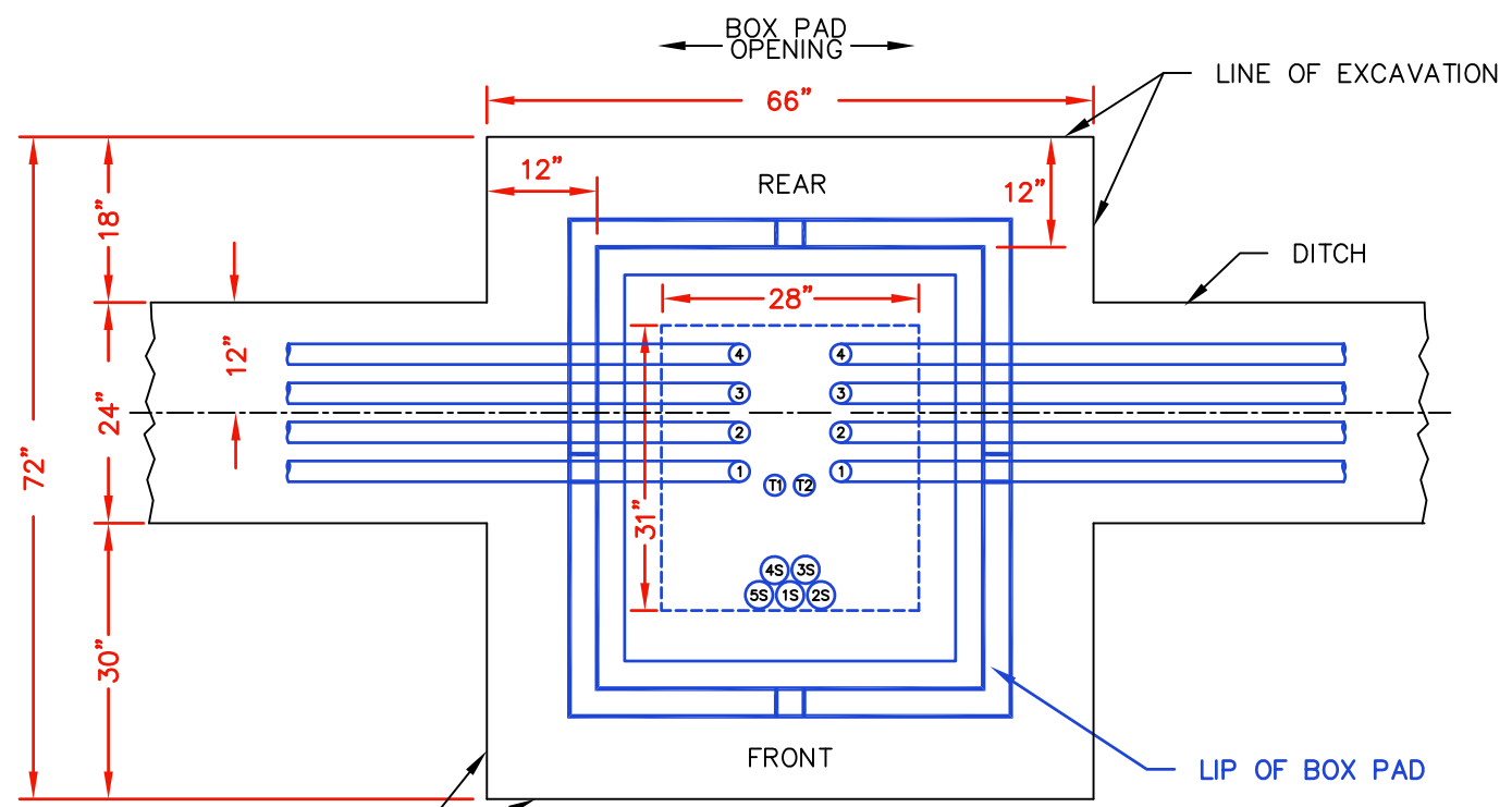
BOX PAD BASE AND EXCAVATION PLAN
