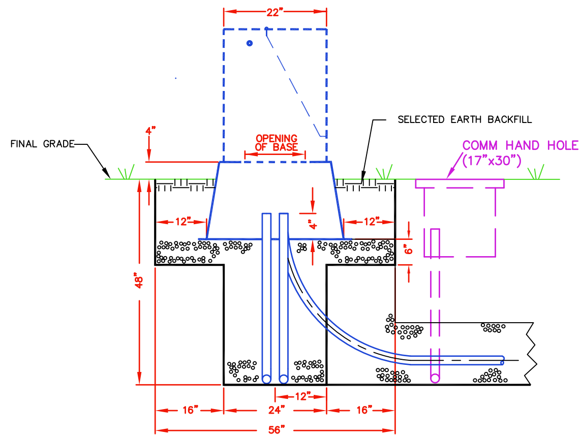
SECTOR SIDE ELEVATION
