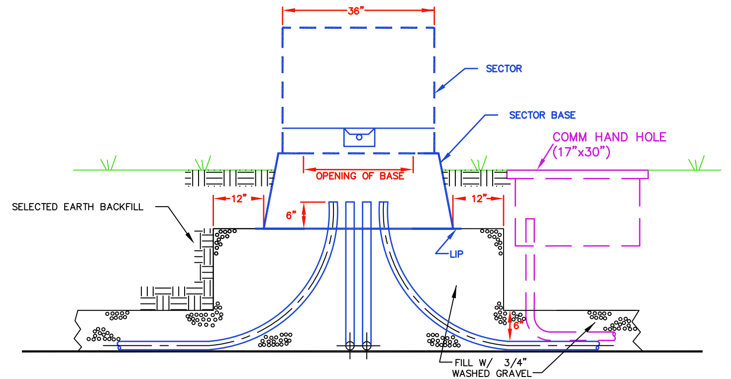
SECTOR FRONT ELEVATION
