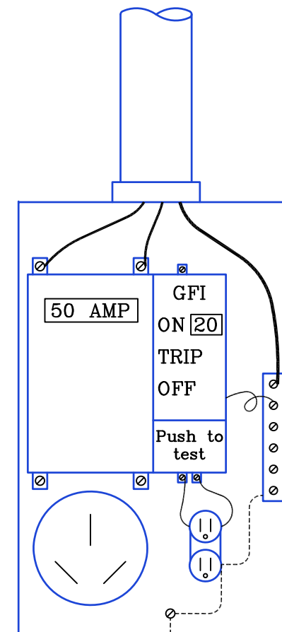
Receptacles SEE NOTE 11 SERVICE PANEL
