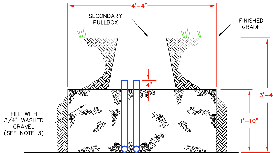
FRONT VIEW
