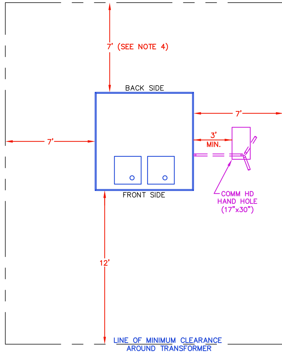
CLEARANCES
