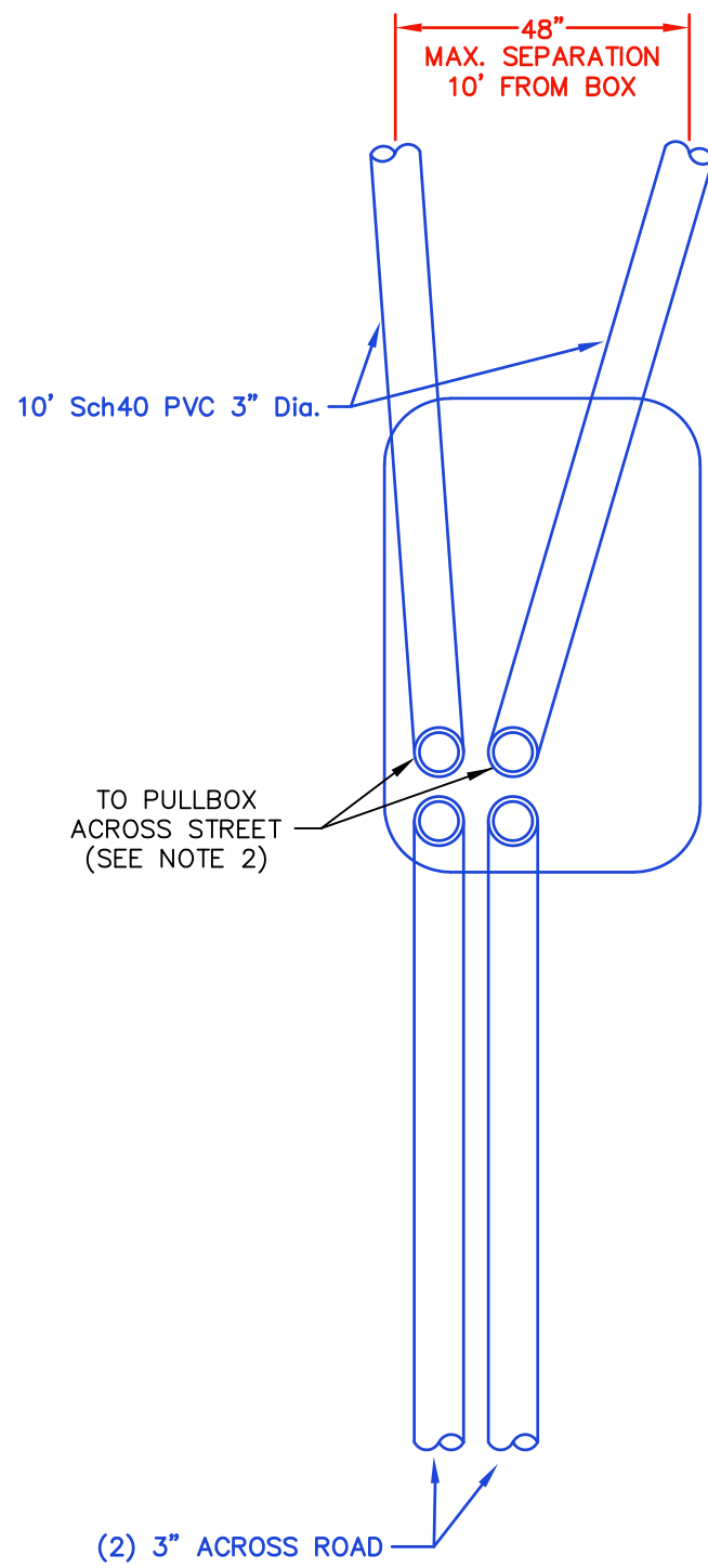
PLAN VIEW SCALE: NONE
