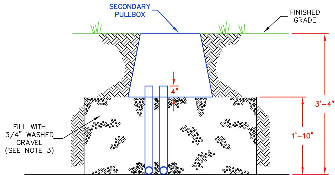
FRONT VIEW SCALE: NONE
