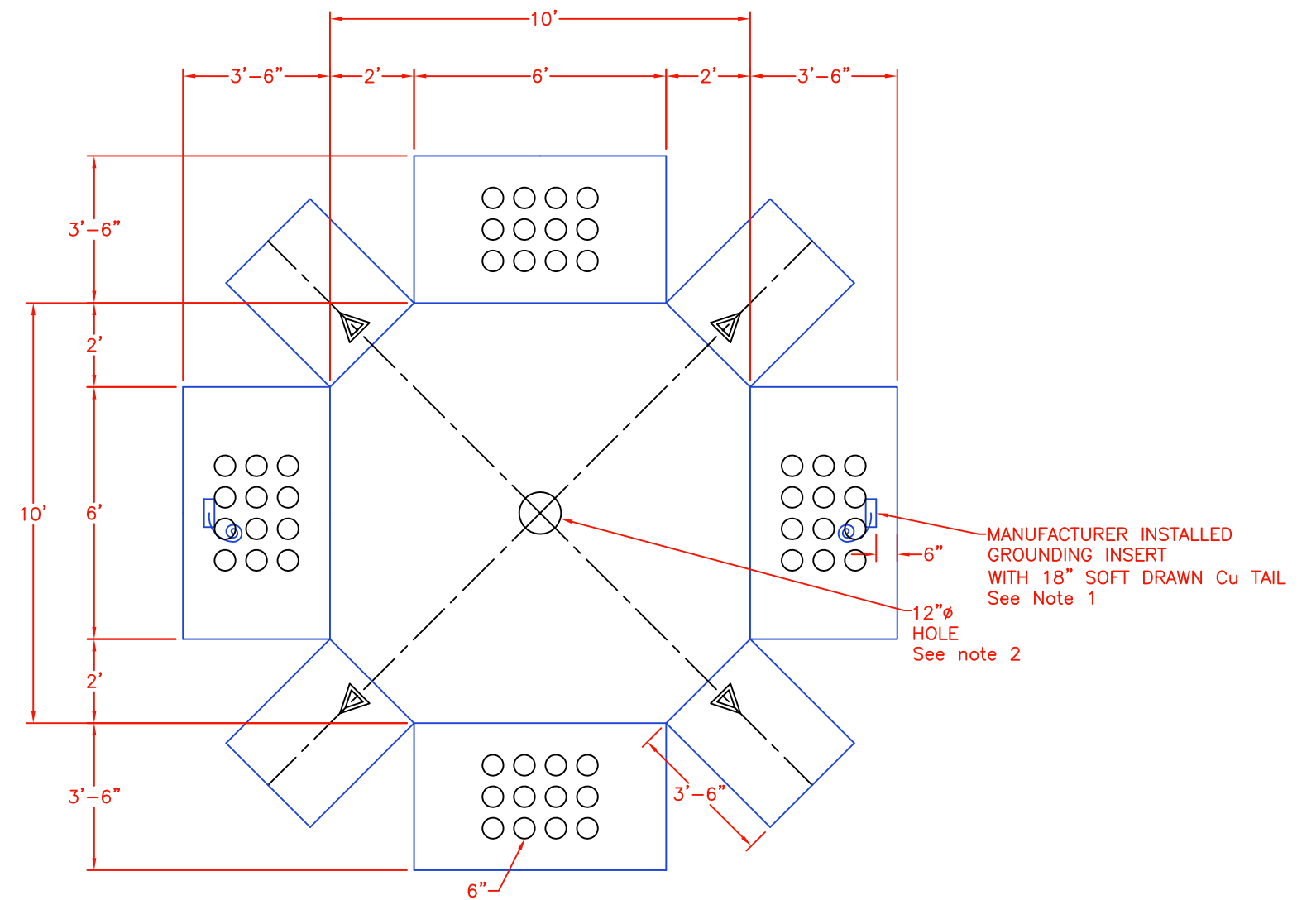
BOTTOM VIEW
