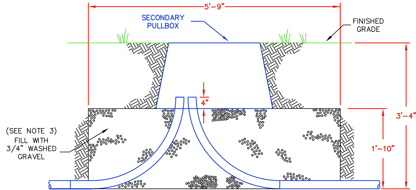
SIDE VIEW
